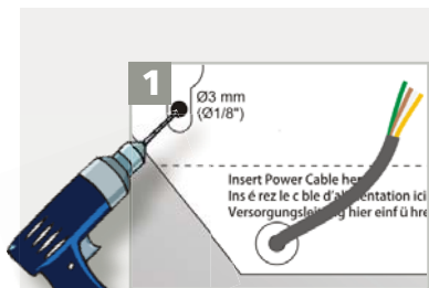
Wall mounting above sliding or revolving door
